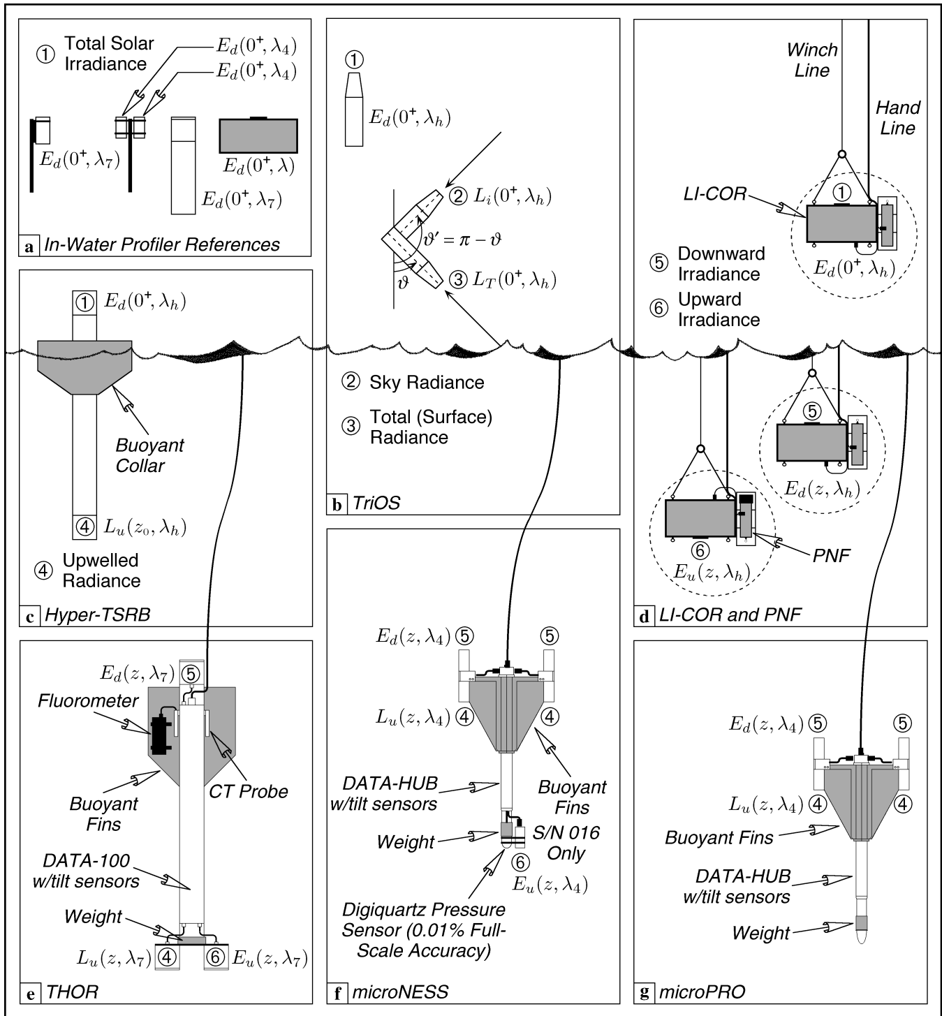
Fig. 3. The AOP instruments deployed during the BENCAL cruise: a) the solar references for the profiling systems, b) the Saturn above-water TriOS radiometers, c) the UCT H-TSRB, d) the LOV LI-COR and PNF radiometers, e) the NASA THOR, f) the NASA microNESS profiler(s), and g) the PML microPRO. The references, from left to right in panel a, correspond to microNESS, microPRO, THOR, and the LI-COR and PNF instruments. The in-water instruments for the latter are shown in the three configurations (dashed circles) used during data collection: incident solar irradiance (top), downward irradiance (middle), and upward irradiance (bottom). Note, the PNF-300 only acquires radiance data during downward irradiance casts (the sensor is covered during upward irradiance casts). Although not shown explicitly, the microNESS and microPRO profilers had external probes to measure seawater temperature.
