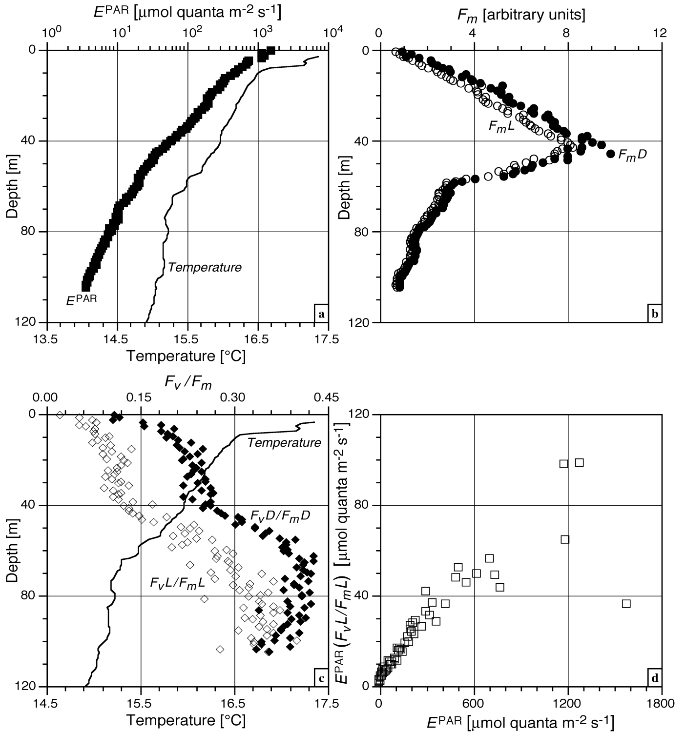
Fig. 12. FRRF profiles to 110 m at station 27 on SDY 286 (13Oct02): a) E^{\text{PAR}} (solid squares) and seawater temperature (solid line); b) fluorescence F_mD (solid circles) and F_mL (open circles); c) F_vD/F_mD (solid diamonds), F_vL/F_mL (open diamonds), and seawater temperature (solid line); d) the product of E^{\text{PAR}} and F_vL/F_mL versus E^{\text{PAR}} (open squares).
