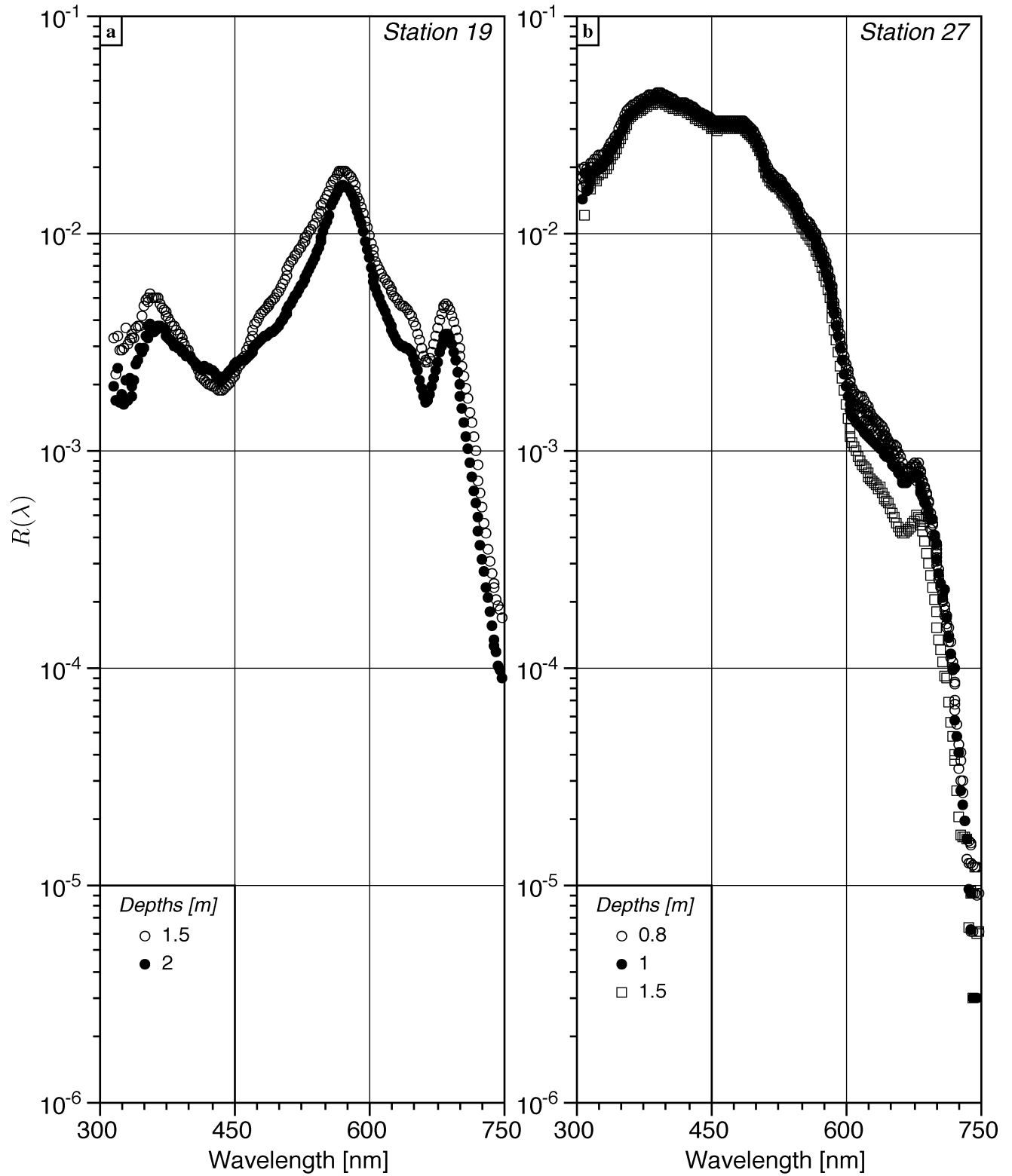
Fig. 6. Reflectance spectra (see text) for the upper layer for the same stations and data presented in Figs. 4 and 5.
