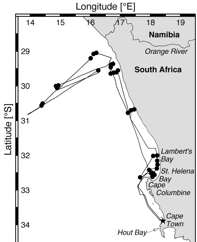
Fig. 1. The BENCAL cruise track (the solid circles are the individual stations).
