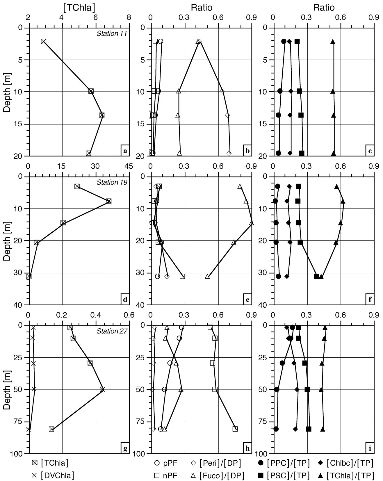
Fig. 7. [TChl a ] and [DVChl a ] (in units of milligrams per cubic meter), diagnostic ratios, and pigment ratios for station 11 (a–c, respectively), station 19 (d–f, respectively), station 27 (g–i, respectively). The water depths for the three stations were 38 m, 127 m, and 1,900 m, respectively.
