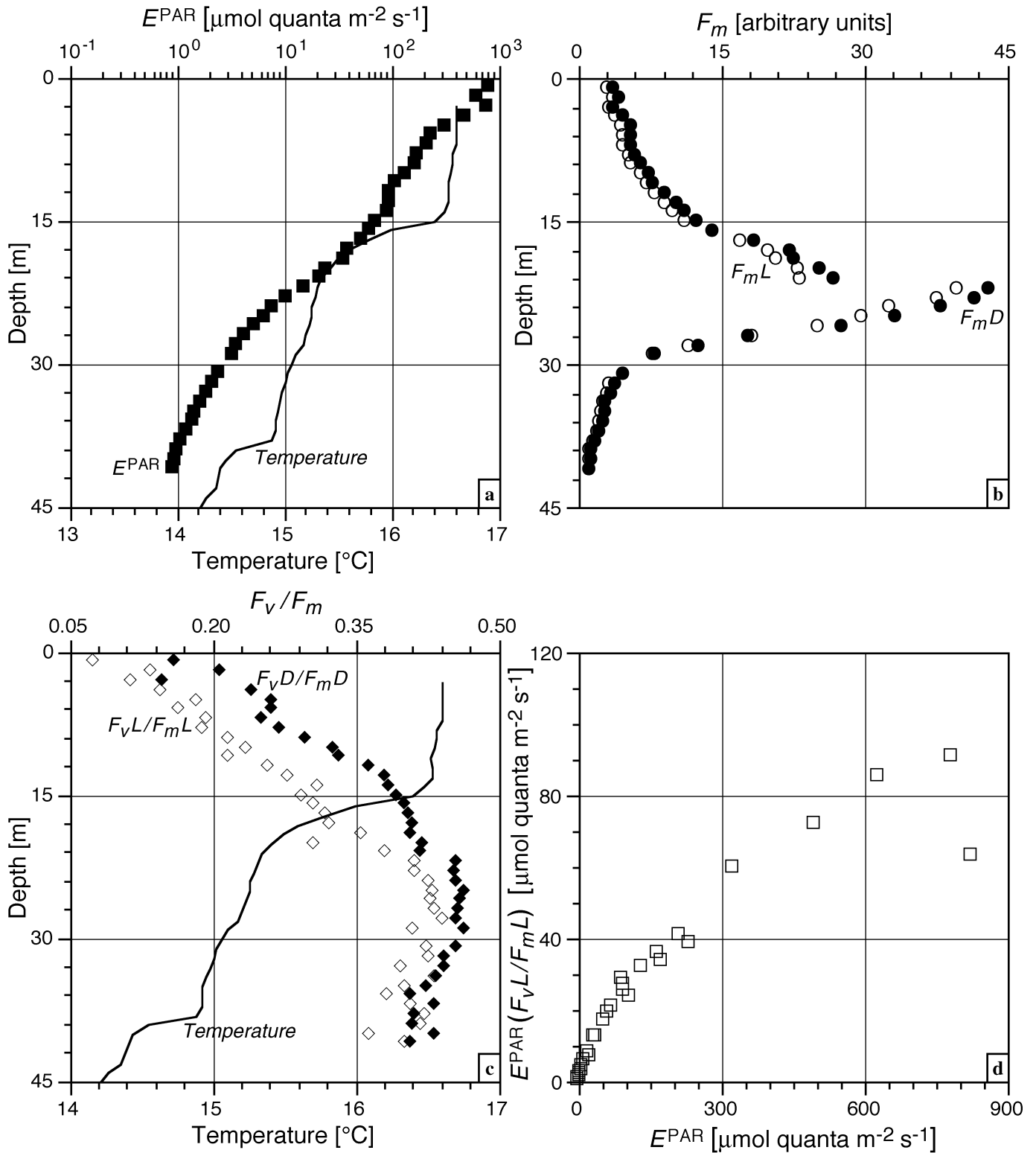
Fig. 13. FRRF profiles to 43 m at station 30 on SDY 287 (14Oct02): a ) E^{\text{PAR}} (solid squares) and seawater temperature (solid line); b ) fluorescence F_m D (solid circles) and F_m L (open circles); c ) F_v D / F_m D (solid diamonds), F_v L / F_m L (open diamonds), and seawater temperature (solid line); d ) the product of E^{\text{PAR}} and F_v L / F_m L versus E^{\text{PAR}} (open squares).
