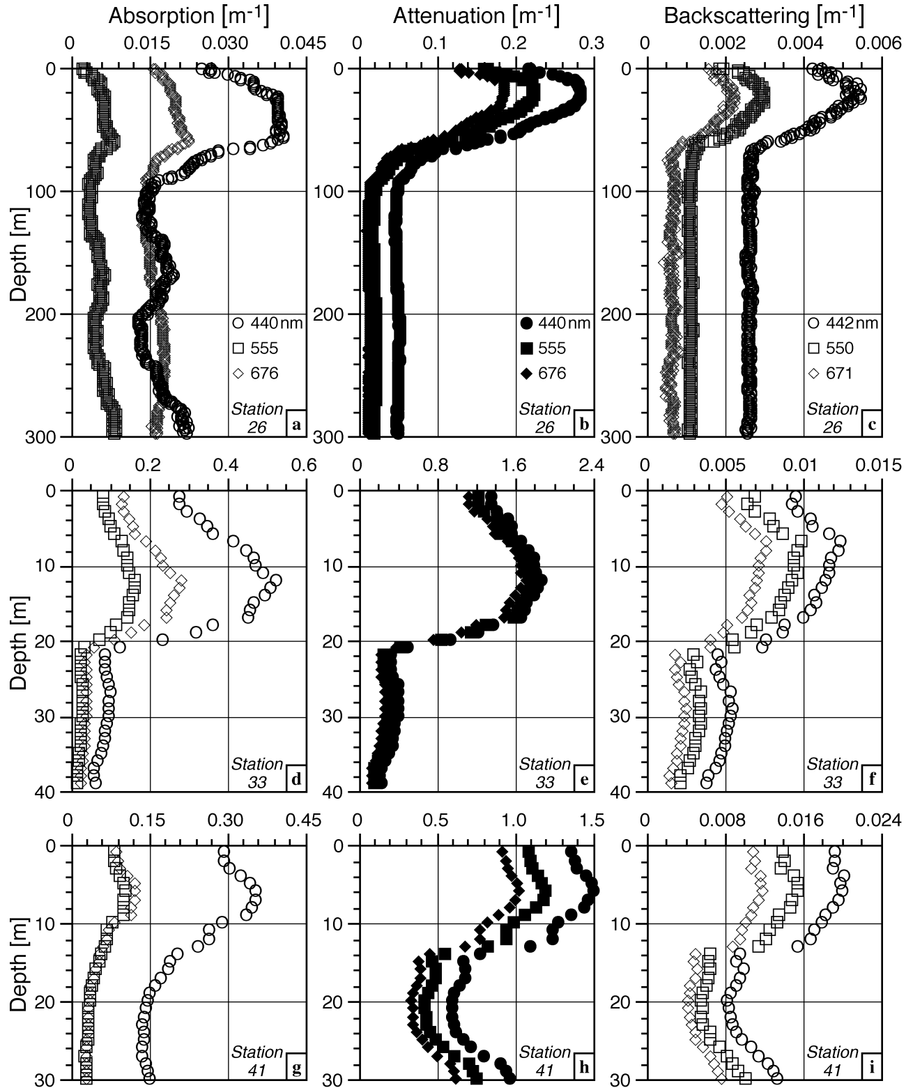
Fig. 10. Vertical profiles of a_T(\lambda) , c_T(\lambda) , b_{bT}(\lambda) for three different stations: 26 (a–c), 33 (d–f), and 41 (g–i), respectively.
