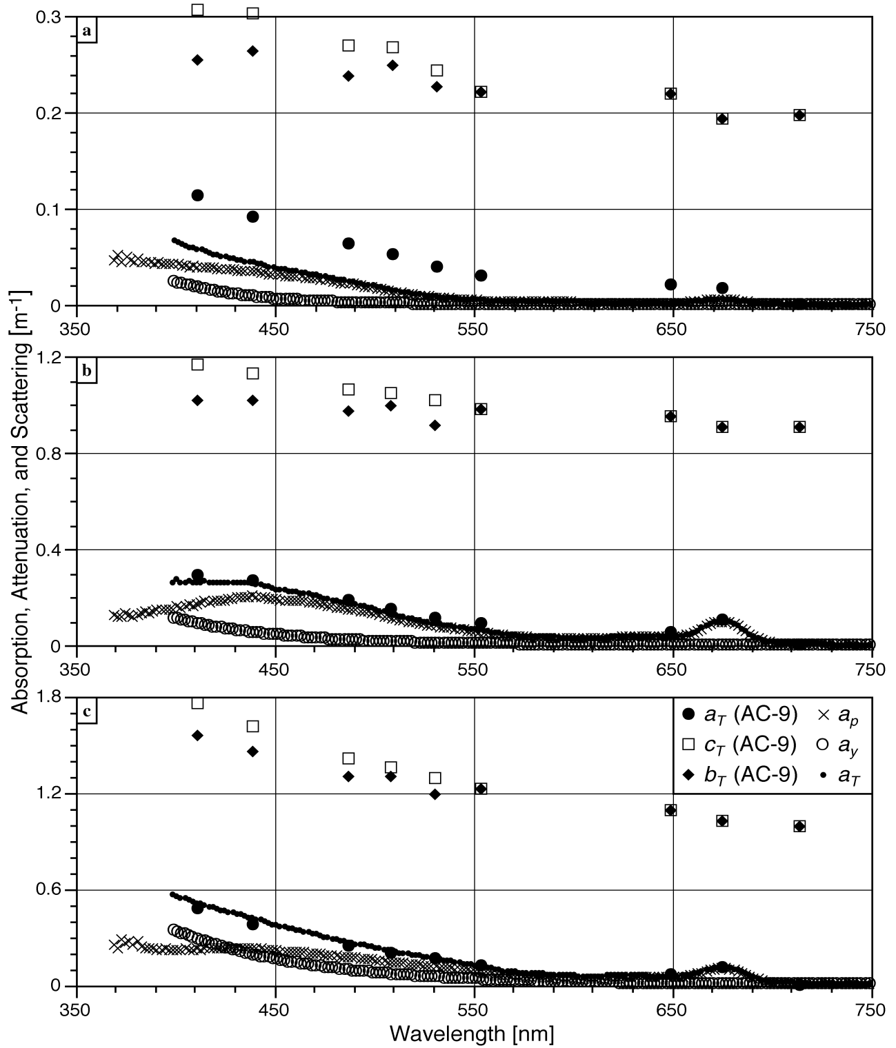
Fig. 9. Spectra of total absorption (large solid circles), attenuation (open squares), and scattering (solid diamonds) from bench-top AC-9 measurements, in addition to particulate absorption (crosses), yellow substance absorption (open circles), and the sum of these two parameters from bench-top spectrophotometric measurements (small solid circles). The analyses are from surface sampling for the following example stations: a) 26, b) 33, and c) 41.
