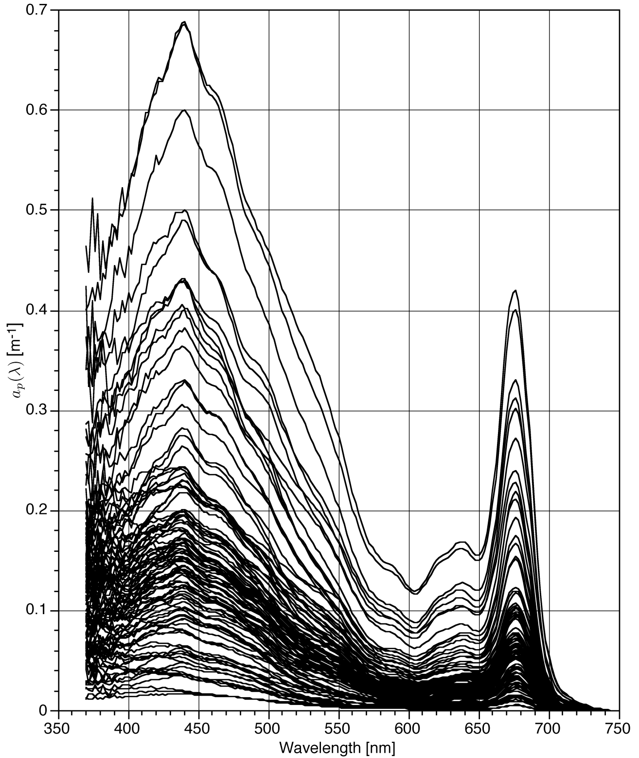
Fig. 11. The absorption coefficient of particulate matter, a_p(\lambda) , between 370–750 nm (in 2 nm increments). The value of a_p(750) is supposed to equal zero, so all other a_p(\lambda) values are shifted accordingly.
