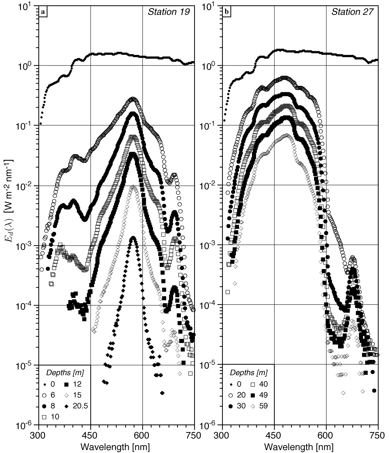
Fig. 4. Downwelling irradiance spectra, E_d(z, \lambda) , at several depths as indicated, for a) station 19 (high chlorophyll a concentration), and b) station 27 (low chlorophyll a concentration). The vertical scale is logarithmic.
