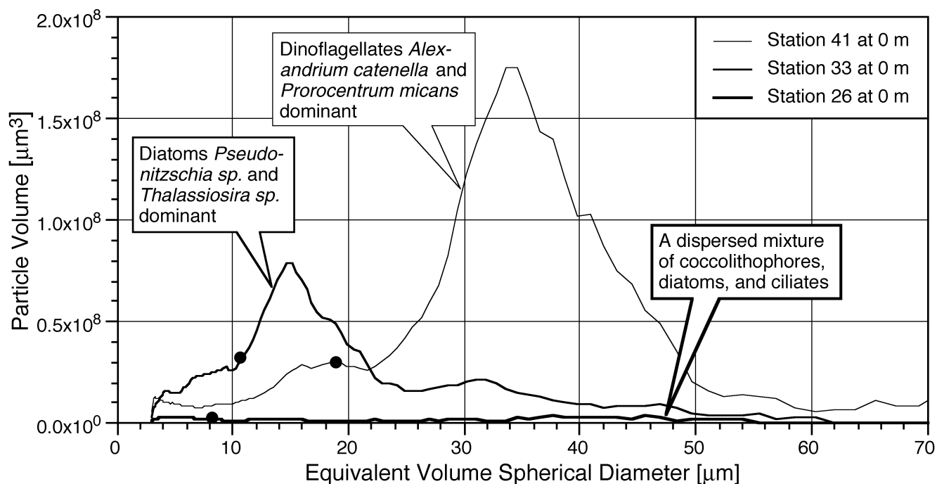
Fig. 8. A plot of the volume PSDs from three sample stations: oligotrophic offshore station 26, diatom-dominated inshore station 33, and dinoflagellate-dominated inshore station 41. Microscopic plankton count data and cell volume calculations are used to identify peaks in the Coulter-measured PSD. Closed circles indicate the effective diameter, 2r_{\text{eff}} , as per (3).
