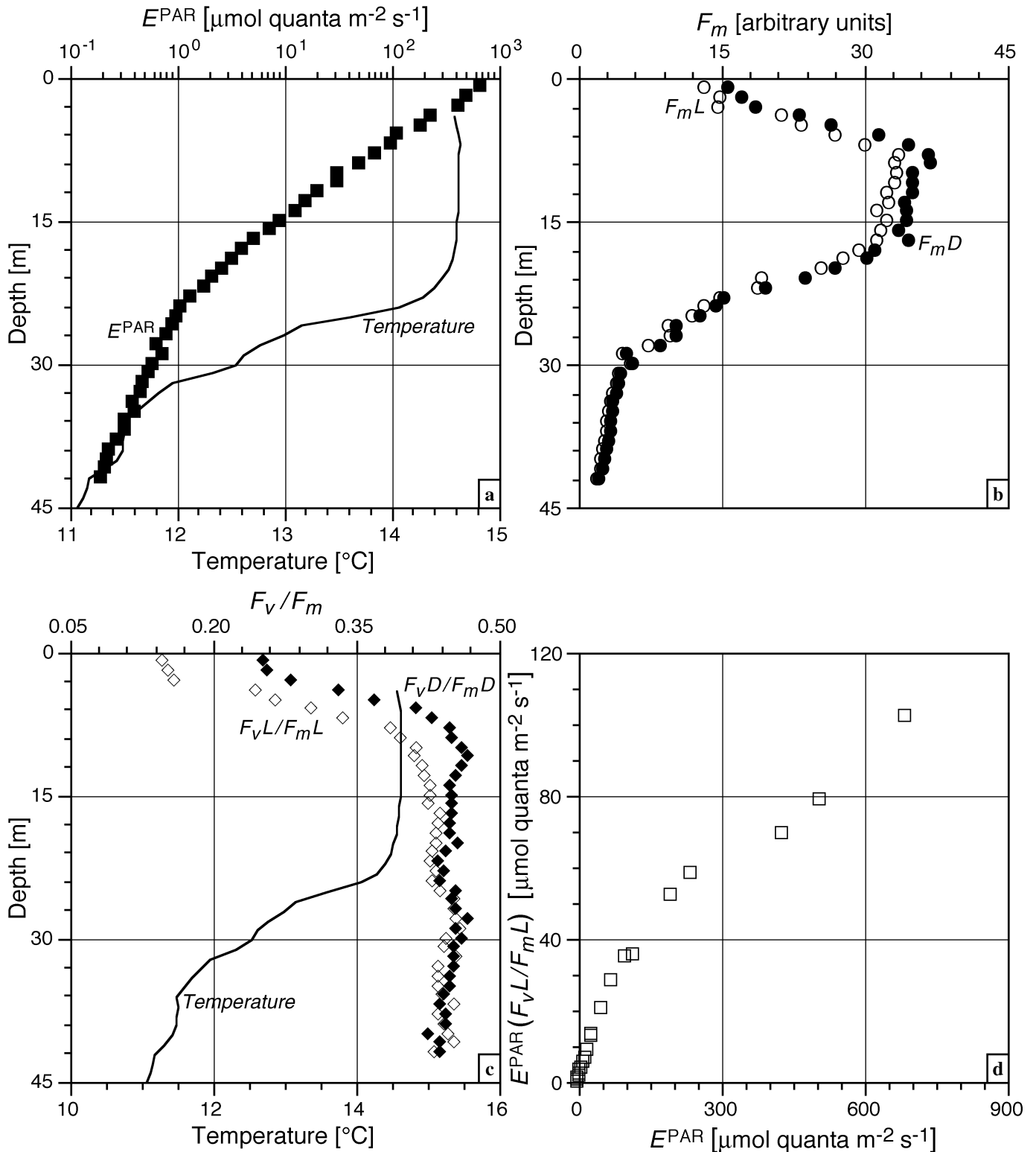
Fig. 14. FRRF profiles to 42 m at station 32 on SDY 288 (15Oct02): a ) E^{\text{PAR}} (solid squares) and seawater temperature (solid line); b ) fluorescence F_mD (solid circles) and F_mL (open circles); c ) F_vD/F_mD (solid diamonds), F_vL/F_mL (open diamonds), and seawater temperature (solid line); d ) the product of E^{\text{PAR}} and F_vL/F_mL versus E^{\text{PAR}} (open squares).
