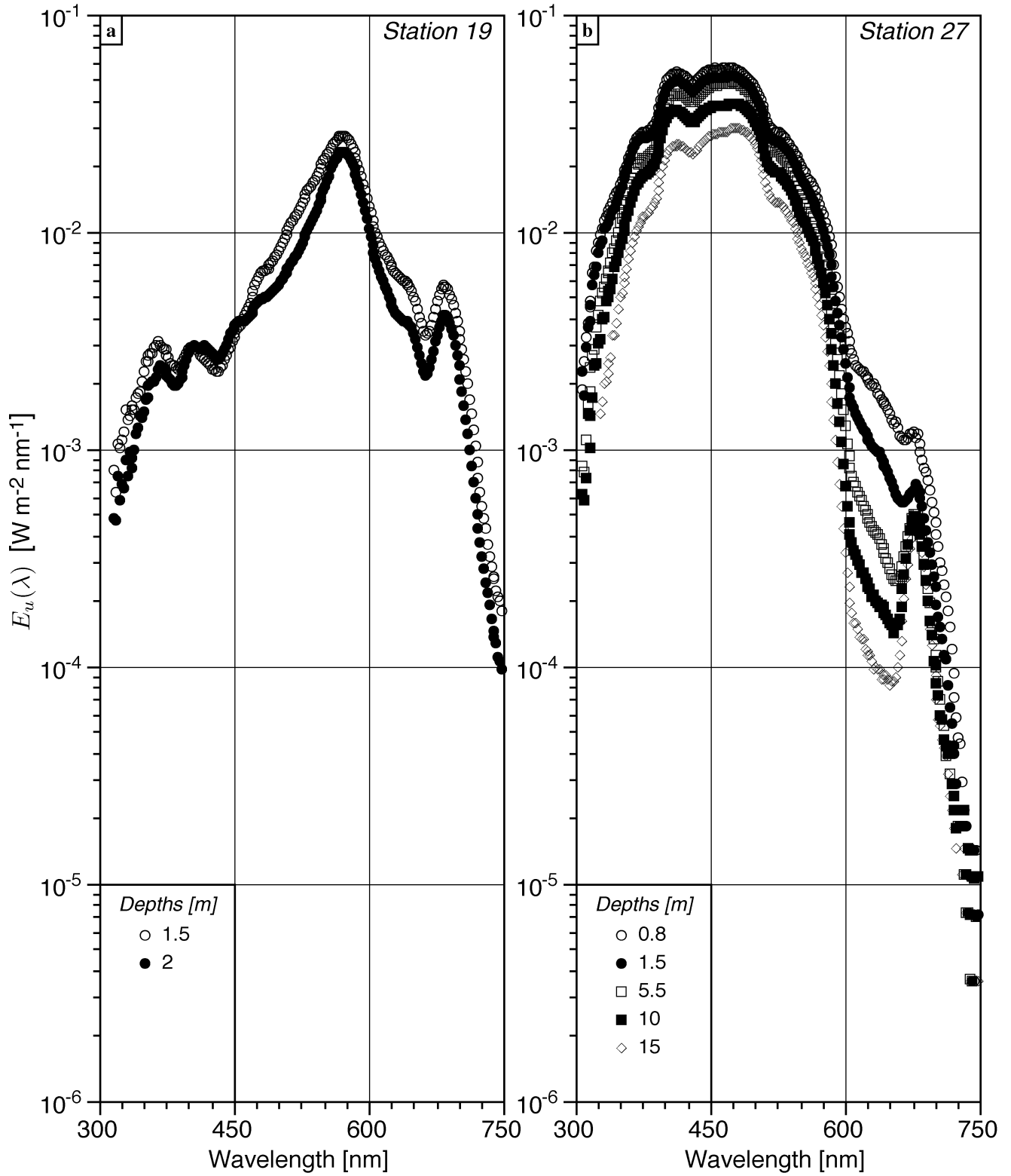
Fig. 5. As in Fig. 4, but for upwelling irradiance, E_u(z, \lambda) . Note, the logarithmic scales are not the same as in Fig. 4.
