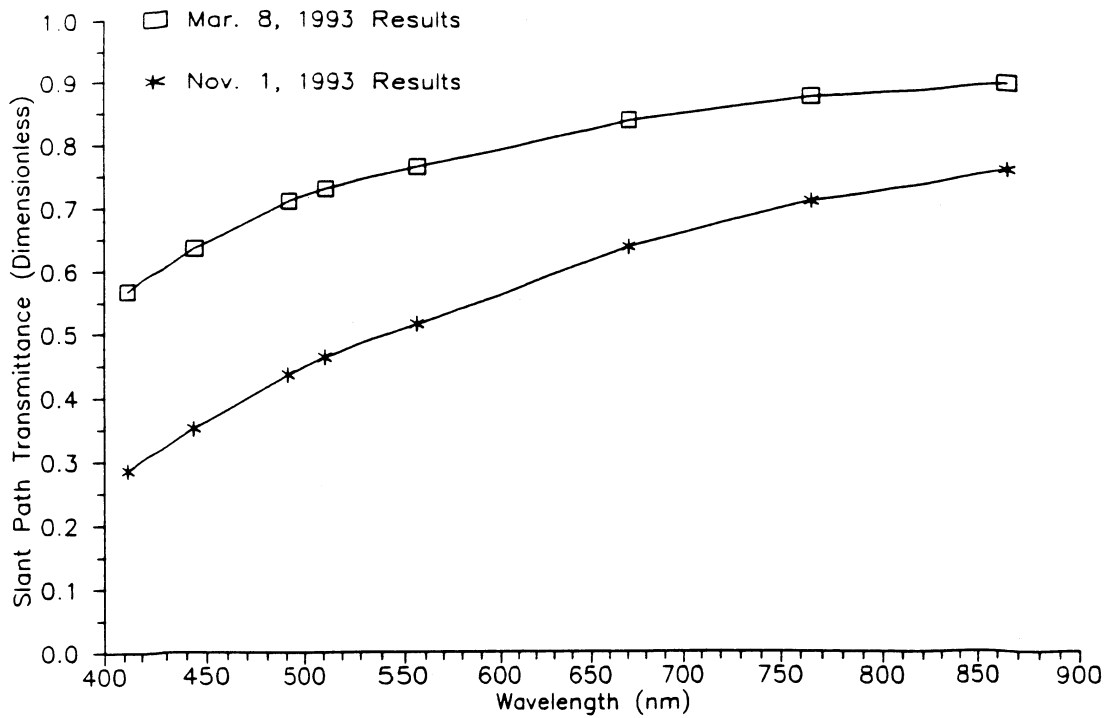
Fig. 11. Measured atmospheric transmittances during the two solar calibration experiments. The transmittances are given at the wavelengths of the Arizona solar radiometer.
