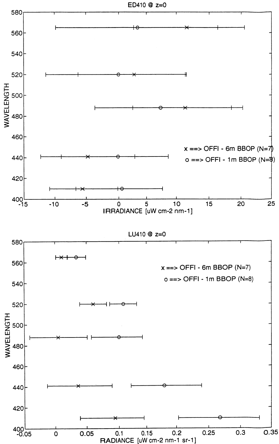
Fig. 16. Mean differences (with 90% c.i.) of simultaneous determinations of the downwelling irradiance spectrum just beneath the sea surface, E_d(0^-, \lambda) , shown in the top panel, and the upwelling radiance spectrum just beneath the sea surface, L_u(0^-, \lambda) , shown in the bottom panel. The differences are between O_{20} casts and B_1 (o; 1 m off the stern) or B_6 (x; 6 m off the stern) BBOP casts.
