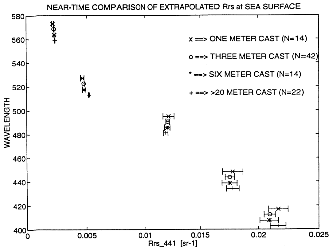
Fig. 18. Spectral structure of the remote sensing reflectance just beneath the sea surface, R_{rs}(0^-, \lambda) , evaluated at four different deployment distances (1, 3, 6, and greater than 20 m).
