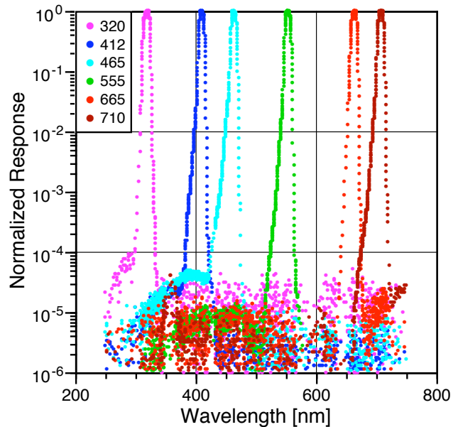
Fig. 4. A semi-log plot of a subset of wavelengths (in nanometers) for the results of the spectral test of the BioSORS irradiance sensor. Features three decades below the peak do not contribute significantly to the measurement.
