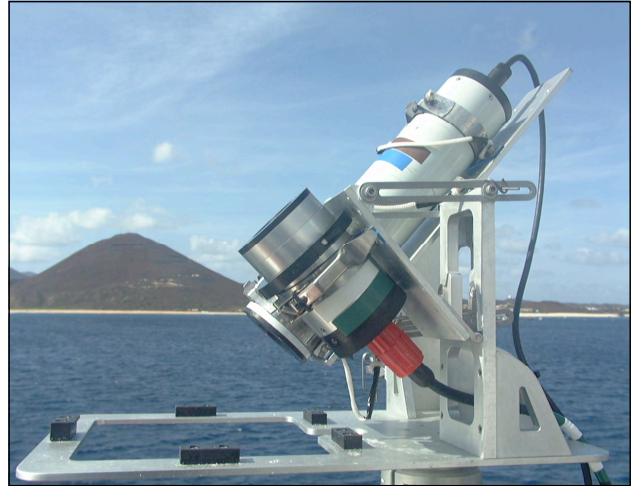
Fig. 2. The SUnSAS frame on the bow of a ship. The long white cylinder is the data logger, which is integral with the L_T (and L_p ) sensor, and the L_i sensor is the smaller silver sensor in the foreground. Both devices are attached to hinged plates that can be secured at the desired viewing angle.
