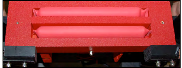
Fig. 42. The C-OPS main buoyancy chamber hollowed out and fitted with two bladders plus a solid foam insert. The removable flotation pieces for adjusting the roll stability of the backplane, with one piece to the left and one to the right, can be seen just below.
