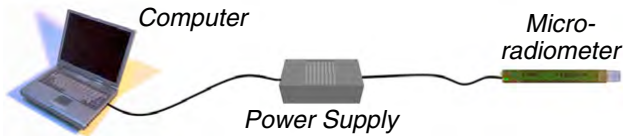
Fig. 26. Individual (or sometimes multiple) microradiometers may be addressed from a computer using a small, external power supply with a communications interface. This is the simplest configuration for single-channel sensors.
