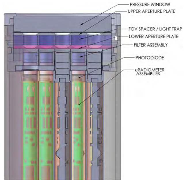
Fig. 36. A cut-away plane view of a 19-channel radiance sensor based on microradiometers.
