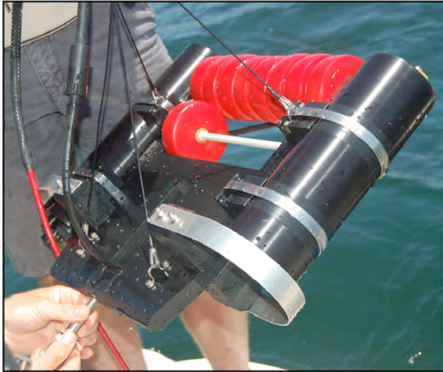
Fig. 14. The early SuBOPS prototype in preparation for redeployment in Mission Bay (California) after having the weighted bottom spar adjusted (not blackened for clarity). Note the aluminum fenders protecting the sensors at the bottom of the profiler (not blackened pending final dimensioning).
