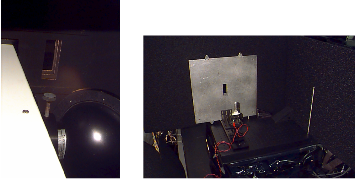
Figure 3.7: Setup at NASA Code 920.1 for FEL measurements with the OL 746. The left picture shows the collecting sphere attached to the OL 746, FEL light enters through a 3-layer baffle. The right picture shows the 3-layer baffle from the other side with the FEL in front of the slit.
