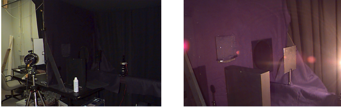
Figure 3.5: Left: SXR-II, fiducial FEL lamp and Spectralon plaque at UCSB. Top left are some of the strings for the curtains that are used to separate this setup from the remaining room. Right: Illuminated FEL lamp at UCSB with two light blocks installed along the optical axis: one on a post, the second block seals a hole in the baffling wall.
