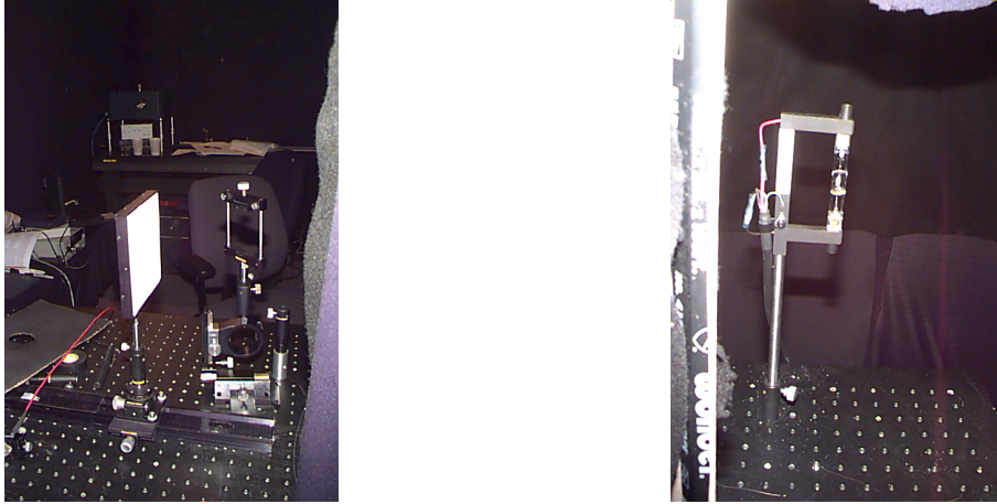
Figure 3.6: Left picture: Spectralon plaque on an optical rail at Hobilabs. The ORIEL lamp is situated on the right of the picture. A sphere can be seen in the background. The picture on the right shows an ORIEL lamp in its mount after removing the baffles between the lamp and the Spectralon plaque.
