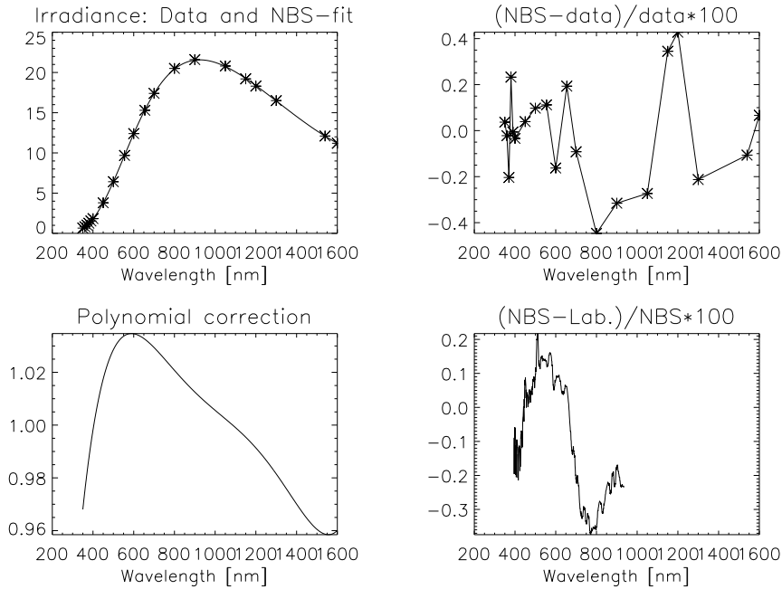
Figure 4.13: Irradiance interpolation comparison for F-400 from NRL. NRL uses Lagrange interpolation. The top left plot shows the calibration points as stars, the solid line is the fit with the NBS method, calculated by the main author of this study. The top right plot shows the differences in % for calibration points and the fitted curve as stars (solid line is for illustration purposes only). The lower left plot shows the polynomial fitted with the NBS method. The lower right plot shows the differences between the interpolated values calculated by the participating laboratories (in this case NRL) and the NBS method.
