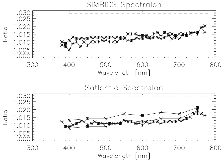
Figure 4.16: Ratios of the BRF R(0^\circ/45^\circ) and the 8^\circ /hemispherical Reflectance Factor from the Labsphere calibrations from August 2001 and September 2001 for the SIMBIOS Spectralon plaque (top). Both ratios increase with wavelength, the August ratio is about 0.002 higher than the September ratio. The lower plot shows the ratio for Spectralon plaques from Satlantic, calibrated by Labsphere in 1995, 1999 and 2001. They increase with wavelength as well, the magnitude of the ratios is also very similar to the SIMBIOS data. The data points are shown as stars, connected by lines.
