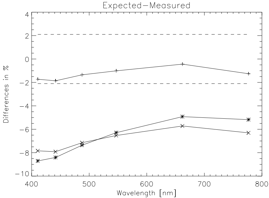
Figure 4.9: Difference of the expected radiance and the SXR-II measured radiance at HOBILabs. +: ORIEL 7-1259, *: ORIEL 7-1244, x: ORIEL 7-1339. The dashed line shows the uncertainty estimate from HOBILabs.
