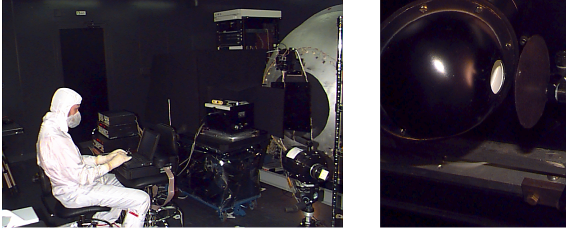
Figure 3.8: Left picture: GSFC Hardy sphere (made of fiberglass, painted a silvery color on the right), aperture covered for FEL measurements. Above the covered aperture the internal monitor can be seen. For Hardy measurements, the OL 746 (in front of the Hardy sphere) is rotated 90° so that the collecting sphere faces the Hardy exit aperture. John Cooper in the white cleanroom suit is using a PC to control the OL 746. Right picture: Collecting sphere of the GSFC 746 with circular disk acting as a block to take ambient measurements.
