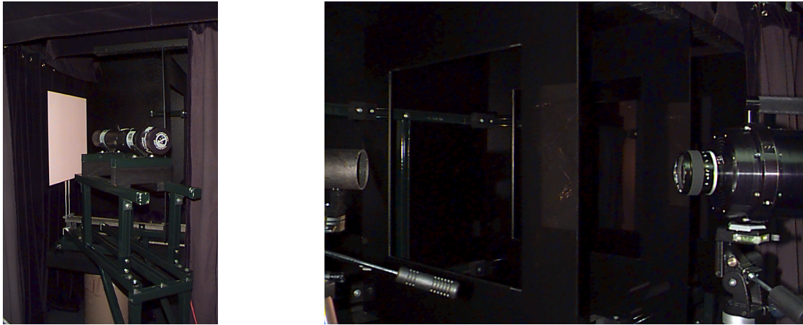
Figure 3.4: Left: Curtains separate measurement area at Biospherical, mechanical mount holds PRR800 radiometer at a viewing angle of 45^\circ to the Spectralon plaque. Right: Three baffles perpendicular along the optical axis at Biospherical.
